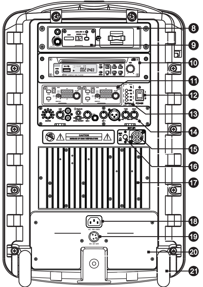
Fig. 2: Rear Panel
